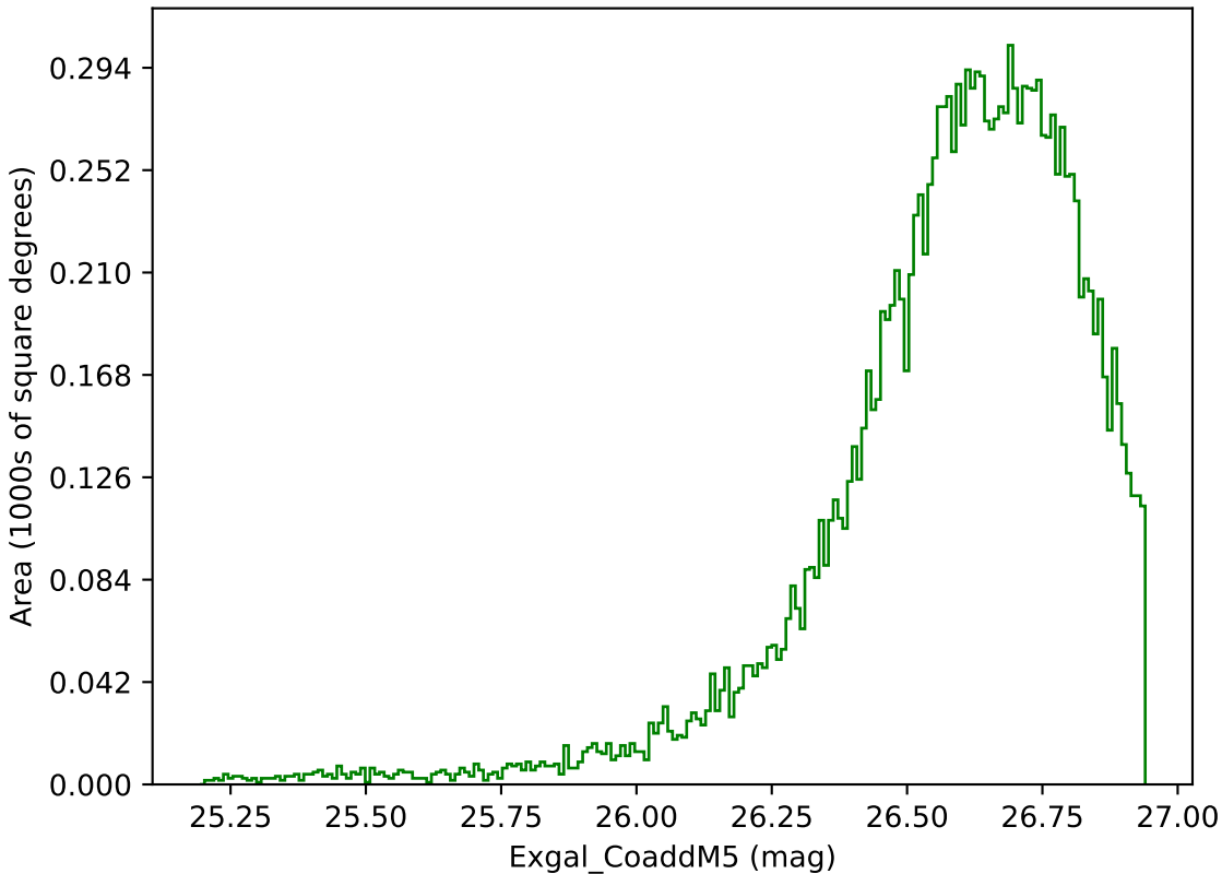
too_elab_r16_d2_ugrizy_v3.4_10yrs WFD g band: Exgal_CoaddM5
