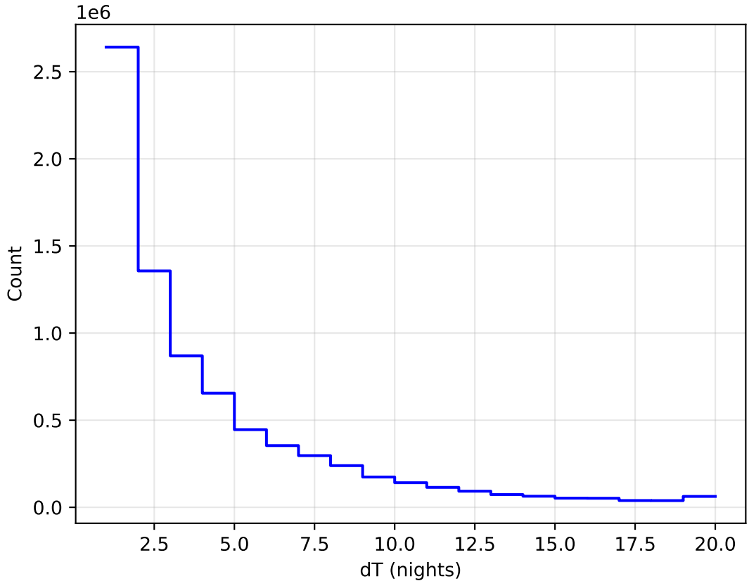
too_elab_r16_d2_ugrizy_v3.4_10yrs WFD all bands: DeltaNight Histogram
