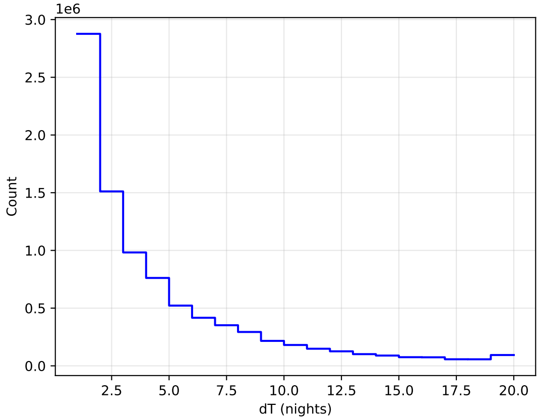
too_elab_r16_d2_ugrizy_v3.4_10yrs All sky all bands: DeltaNight Histogram
