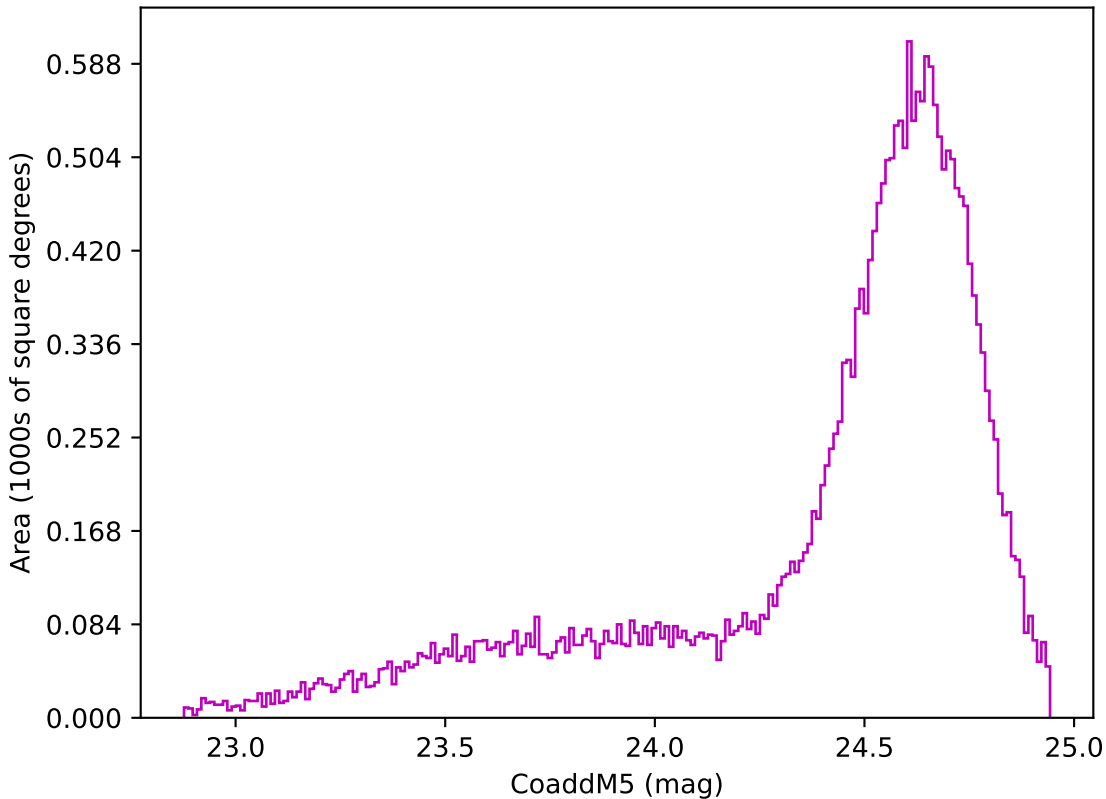
too_elab_r16_d2_ugrizy_v3.4_10yrs Yr 1 z band: CoaddM5
