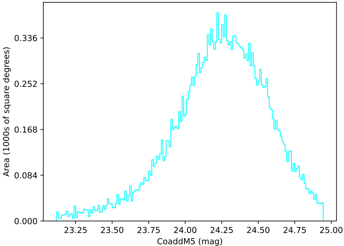
too_elab_r16_d2_ugrizy_v3.4_10yrs Yr 1 u band: CoaddM5
