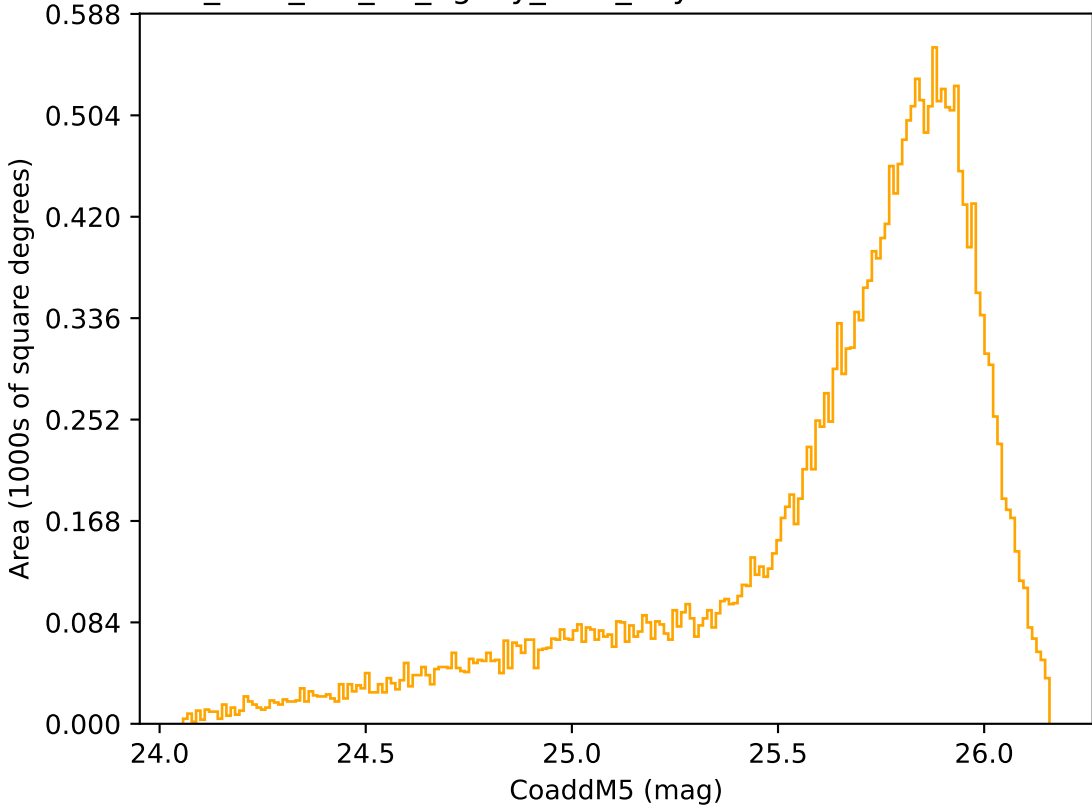
too_elab_r16_d2_ugrizy_v3.4_10yrs Yr 1 r band: CoaddM5
