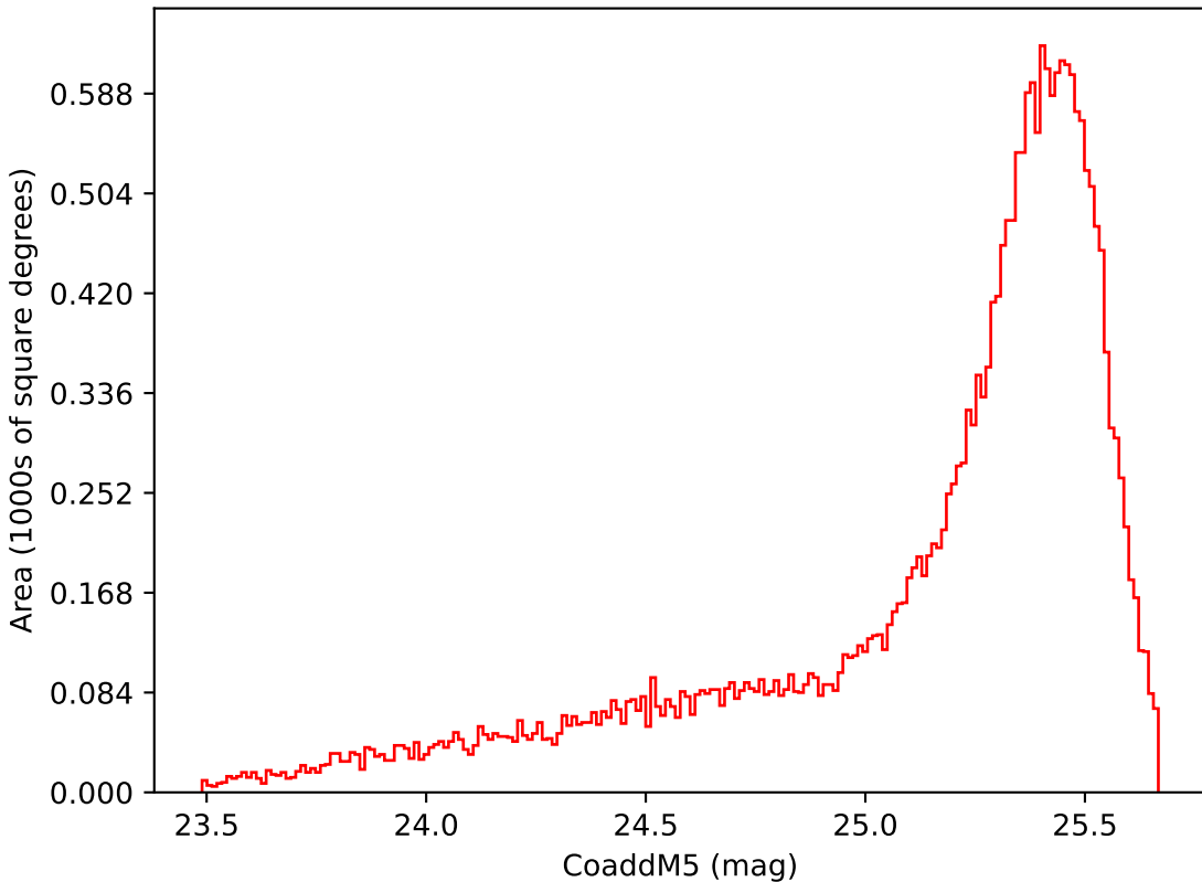
too_elab_r16_d2_ugrizy_v3.4_10yrs Yr 1 i band: CoaddM5
