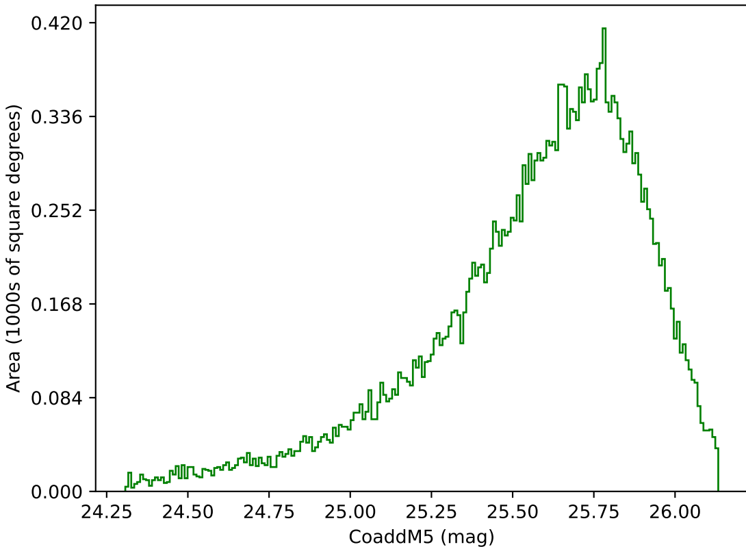
too_elab_r16_d2_ugrizy_v3.4_10yrs Yr 1 g band: CoaddM5
