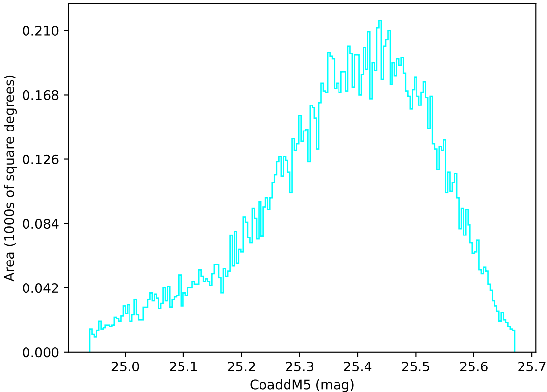
too_elab_r16_d2_ugrizy_v3.4_10yrs WFD u band: CoaddM5
