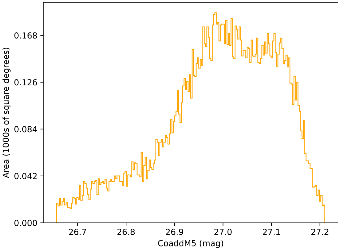
too_elab_r16_d2_ugrizy_v3.4_10yrs WFD r band: CoaddM5
