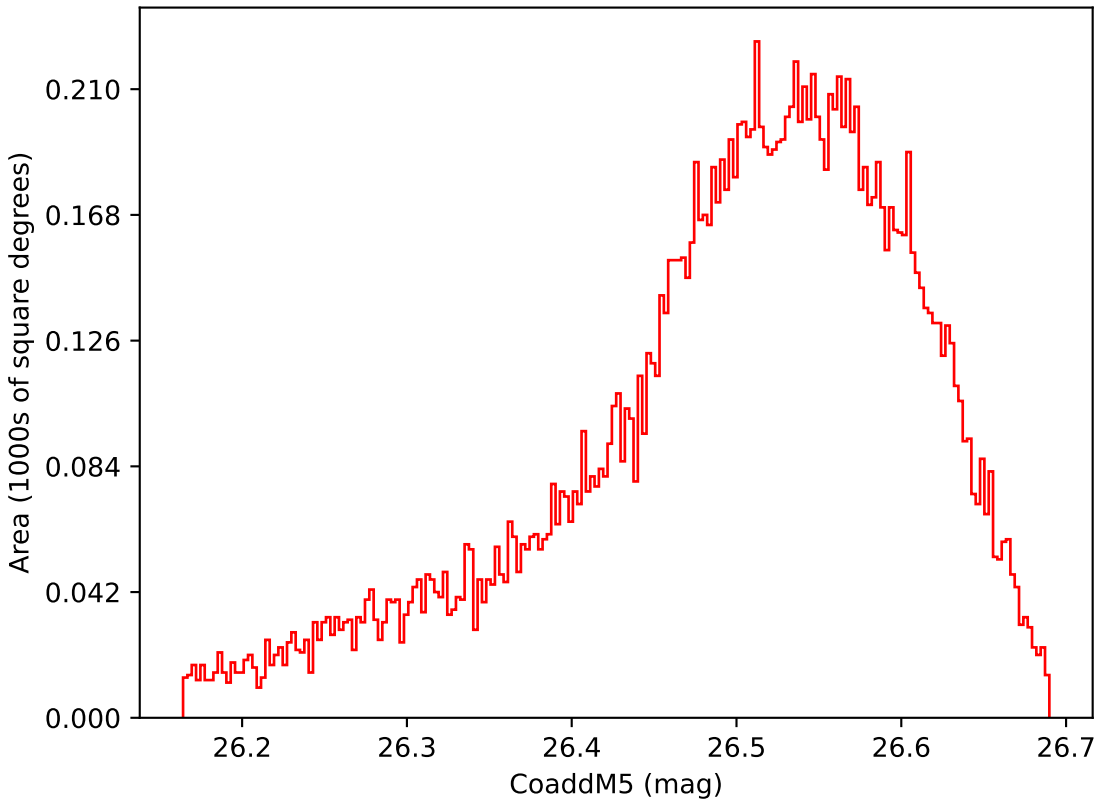
too_elab_r16_d2_ugrizy_v3.4_10yrs WFD i band: CoaddM5
