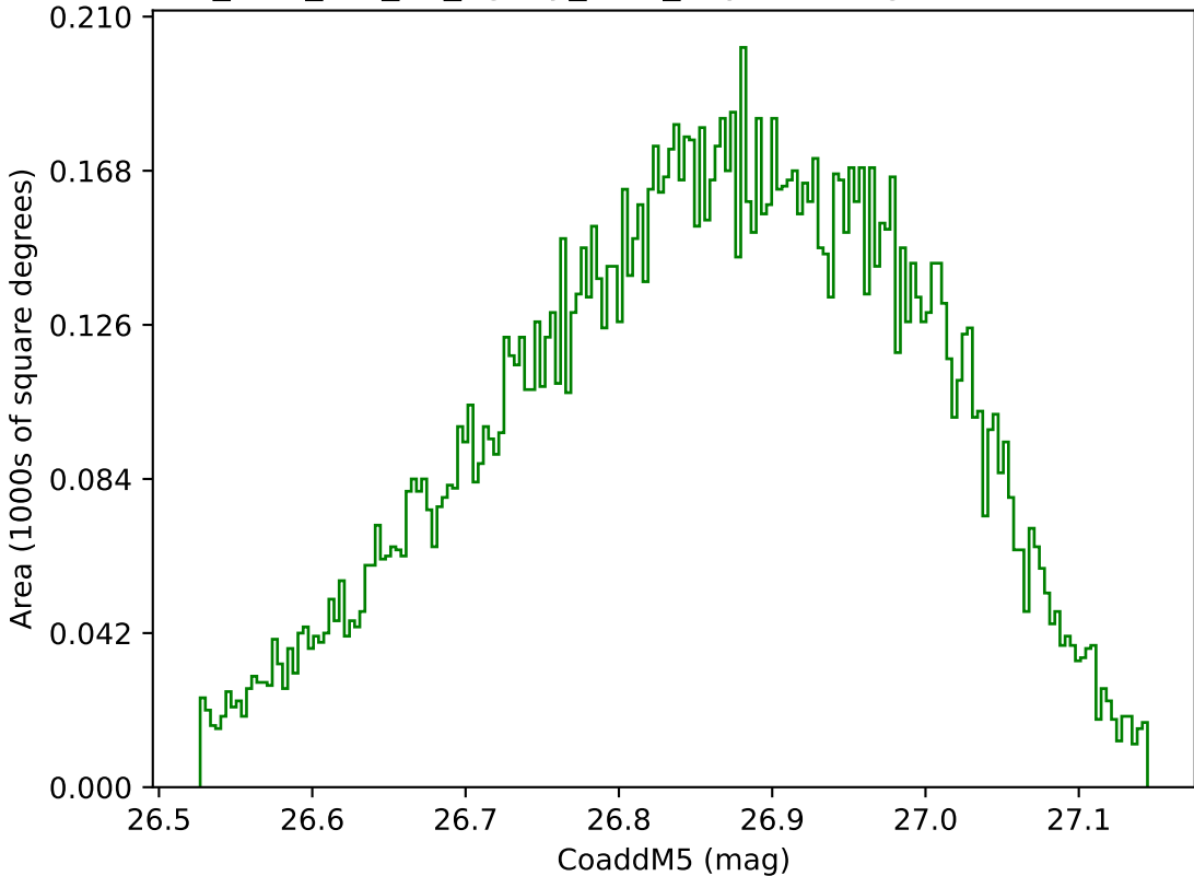
too_elab_r16_d2_ugrizy_v3.4_10yrs WFD g band: CoaddM5
