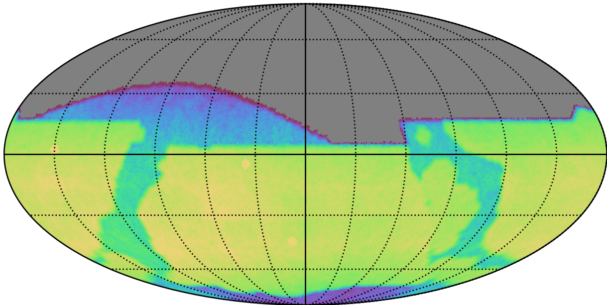
too_elab_r16_d2_ugrizy_v3.4_10yrs All sky z band: CoaddM5
