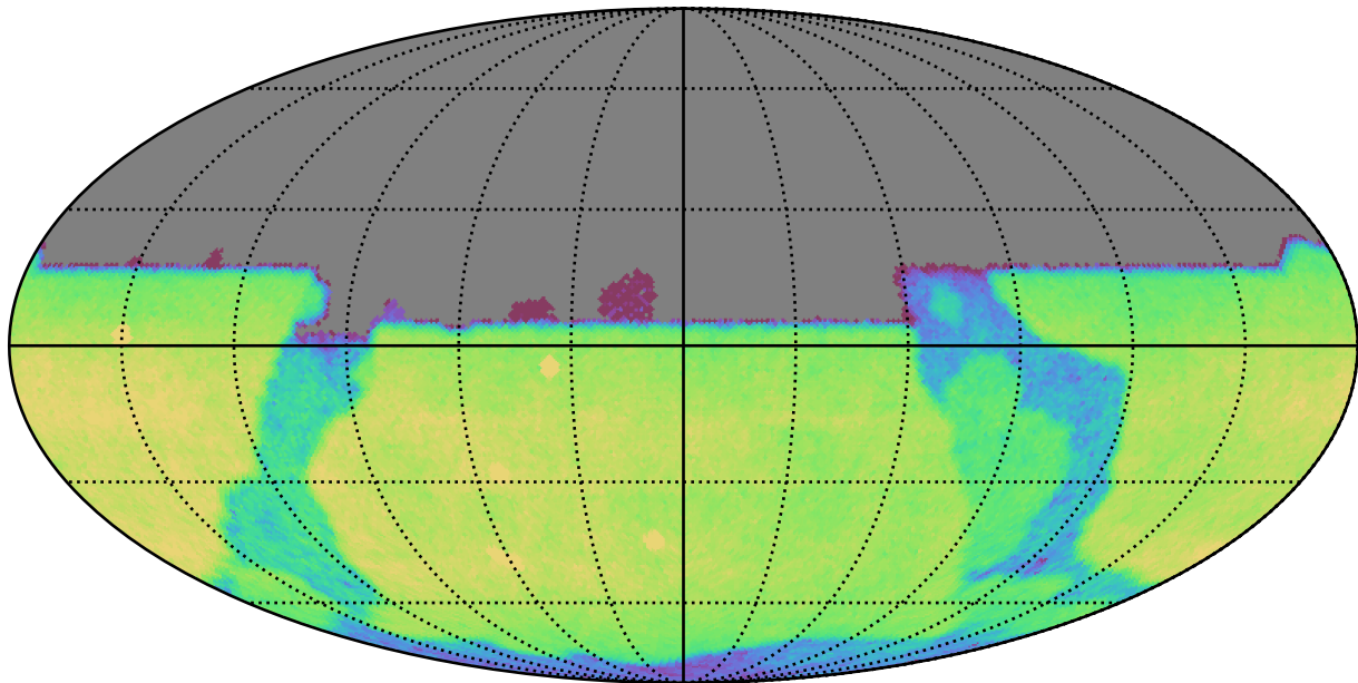
too_elab_r16_d2_ugrizy_v3.4_10yrs All sky u band: CoaddM5
