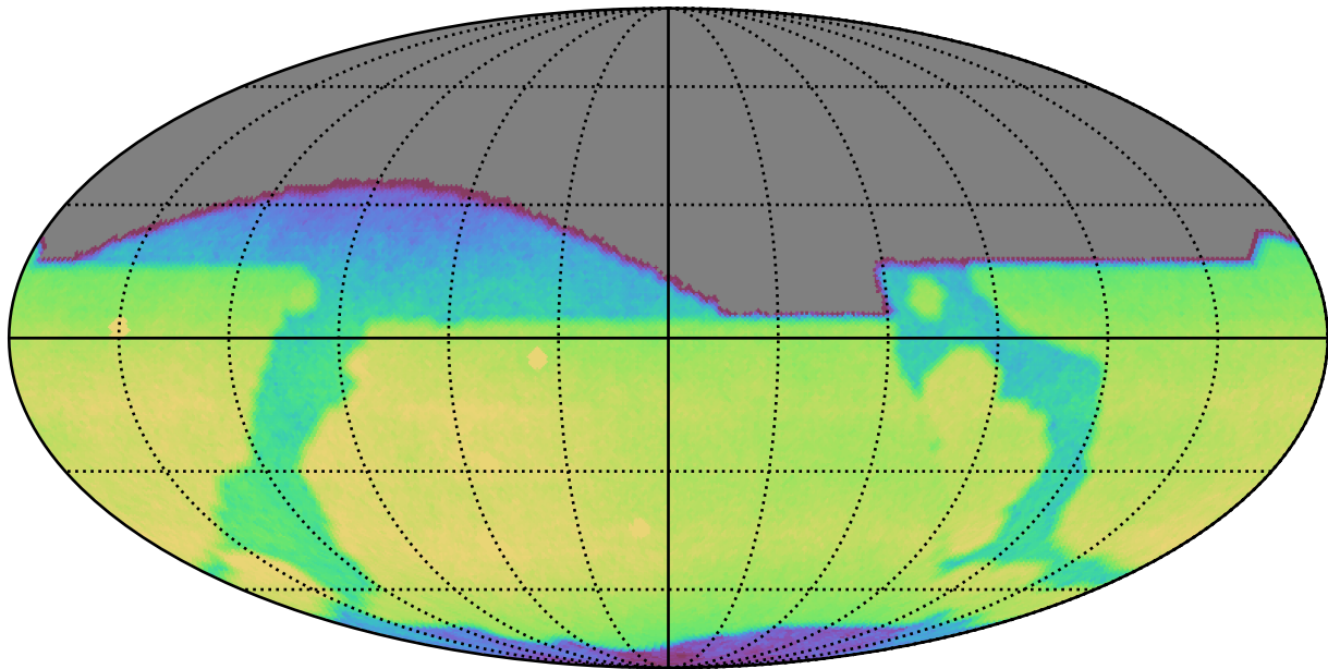
too_elab_r16_d2_ugrizy_v3.4_10yrs All sky r band: CoaddM5
