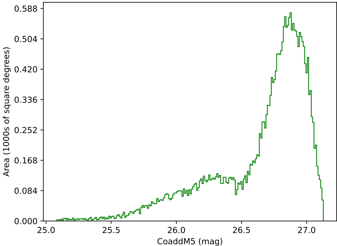
too_elab_r16_d2_ugrizy_v3.4_10yrs All sky g band: CoaddM5
