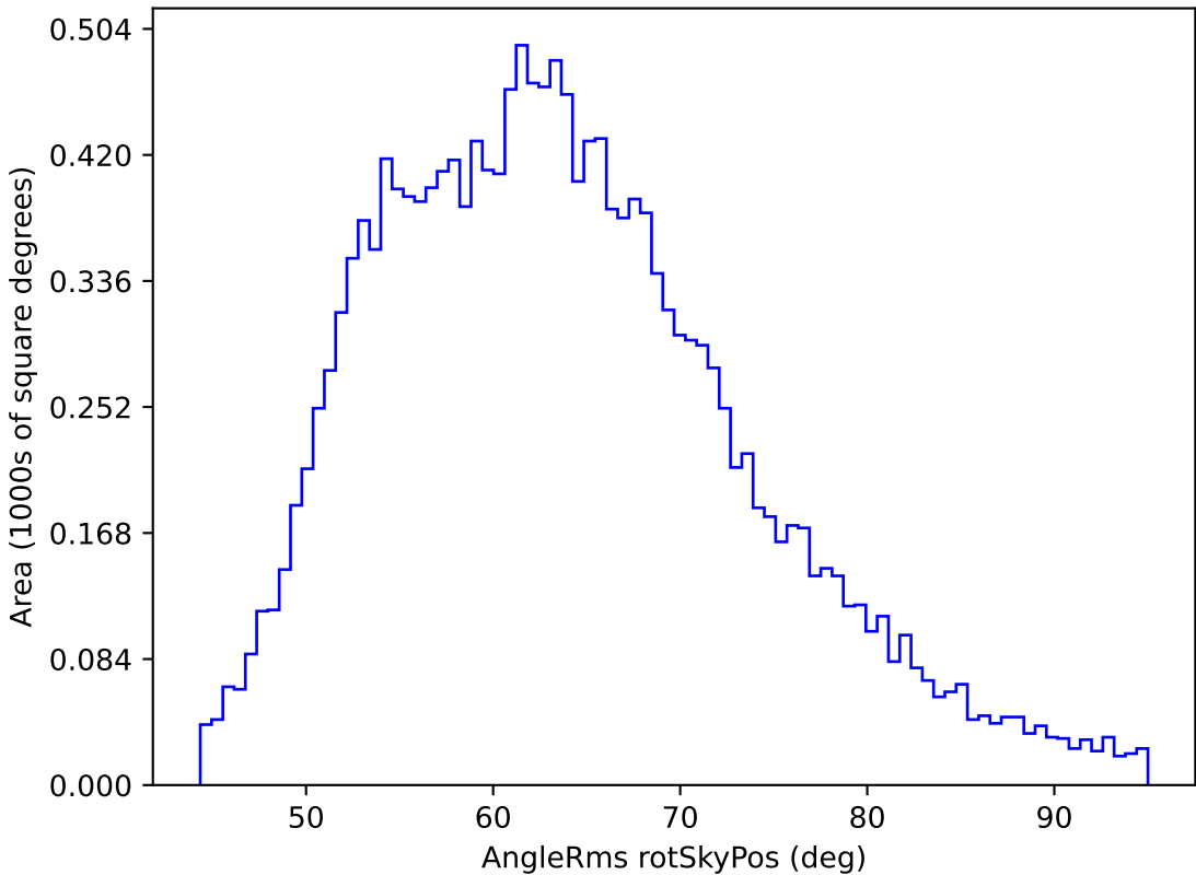
too_elab_r16_d2_ugrizy_v3.4_10yrs WFD u band: AngleRms rotSkyPos
