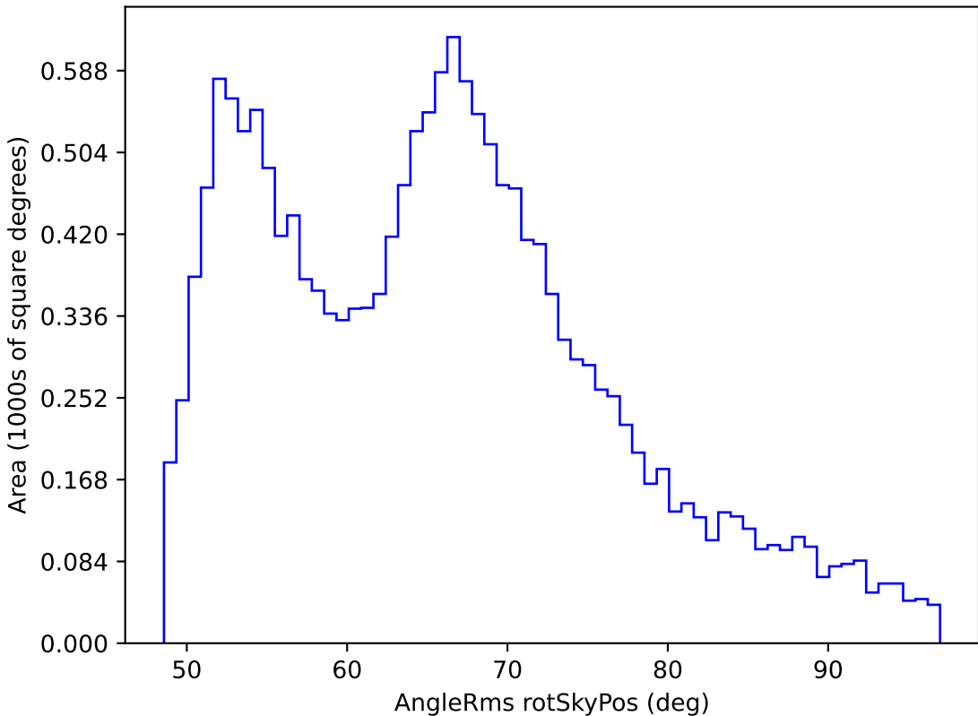
too_elab_r16_d2_ugrizy_v3.4_10yrs WFD r band: AngleRms rotSkyPos
