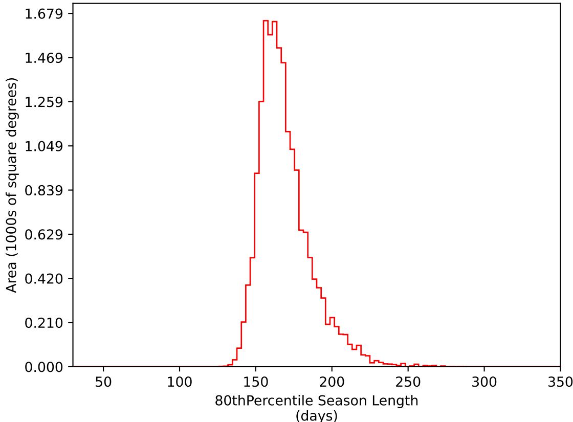
too_elab_r16_d2_ugrizy_v3.4_10yrs WFD i band: 80thPercentile Season Length
