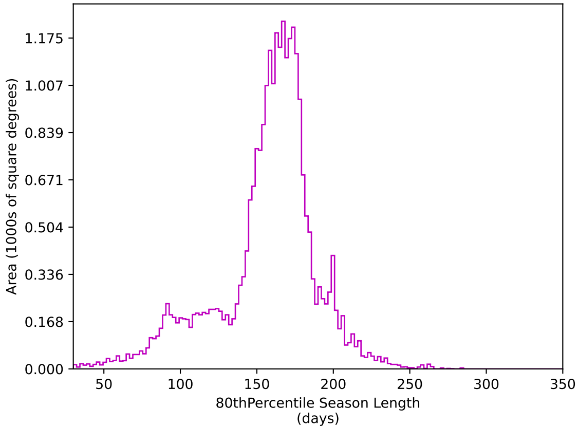
too_elab_r16_d2_ugrizy_v3.4_10yrs All sky z band: 80thPercentile Season Length
