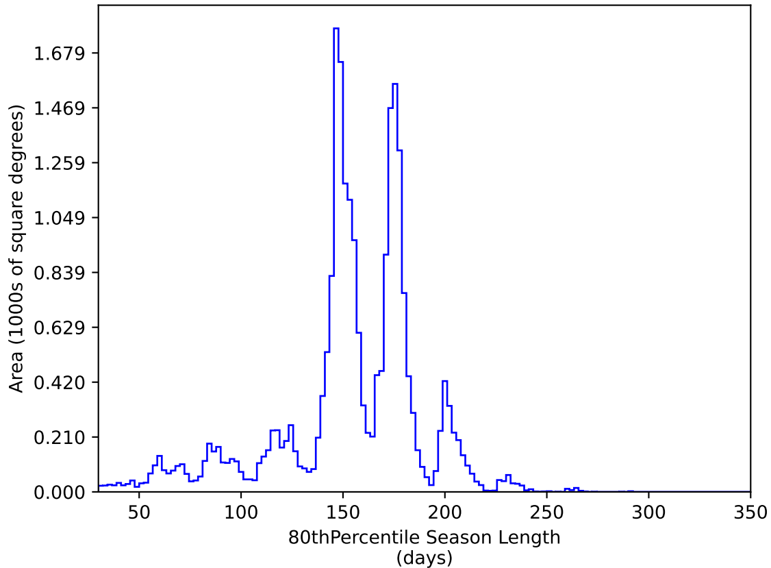
too_elab_r16_d2_ugrizy_v3.4_10yrs All sky y band: 80thPercentile Season Length
