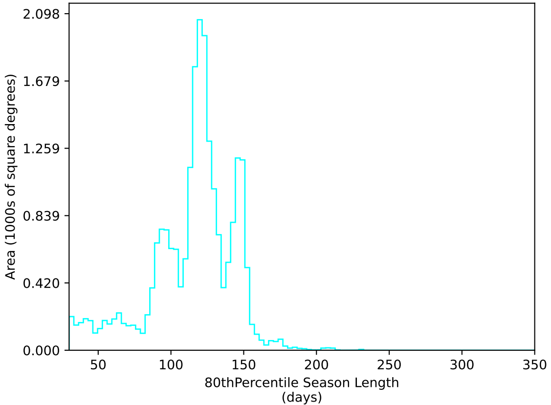
too_elab_r16_d2_ugrizy_v3.4_10yrs All sky u band: 80thPercentile Season Length
