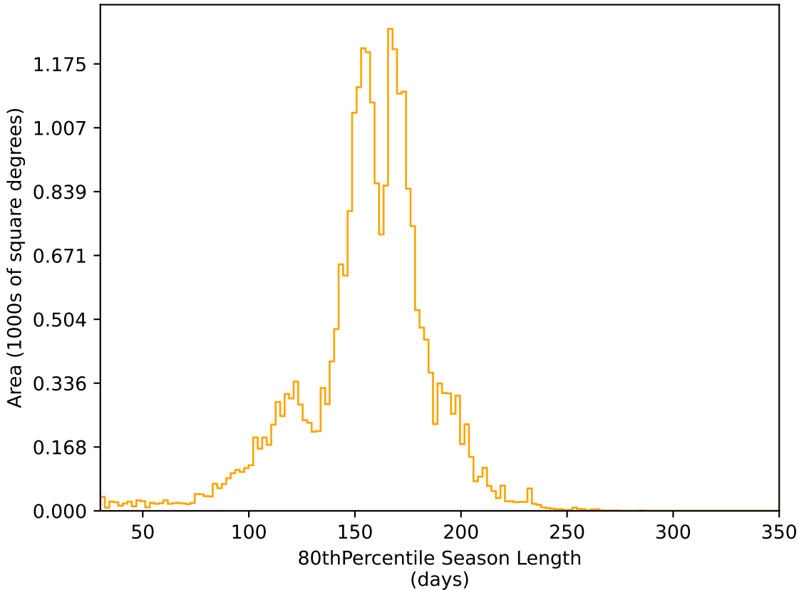
too_elab_r16_d2_ugrizy_v3.4_10yrs All sky r band: 80thPercentile Season Length
