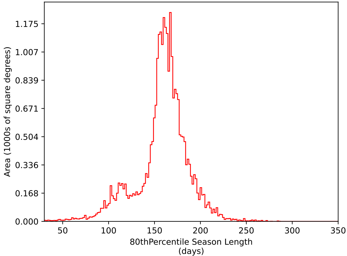
too_elab_r16_d2_ugrizy_v3.4_10yrs All sky i band: 80thPercentile Season Length
