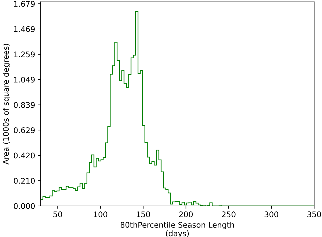
too_elab_r16_d2_ugrizy_v3.4_10yrs All sky g band: 80thPercentile Season Length
