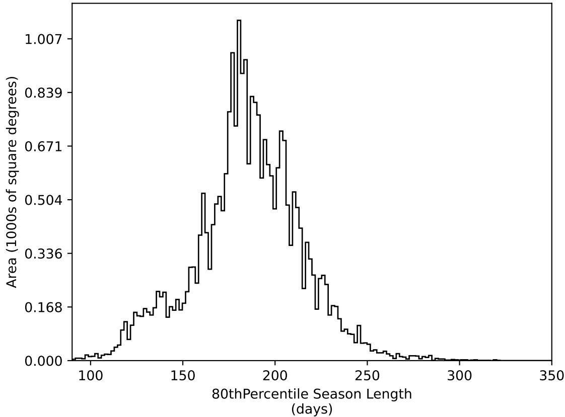
too_elab_r16_d2_ugrizy_v3.4_10yrs All sky all bands: 80thPercentile Season Length
