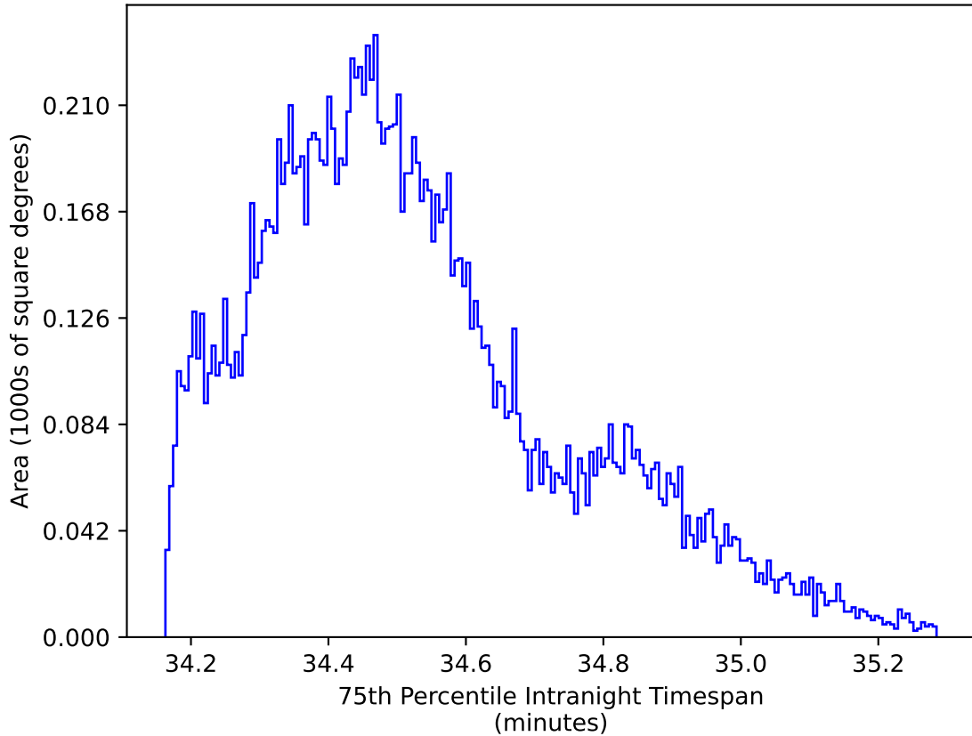
too_elab_r16_d2_ugrizy_v3.4_10yrs WFD zy bands: 75th Percentile Intranight Timespan
