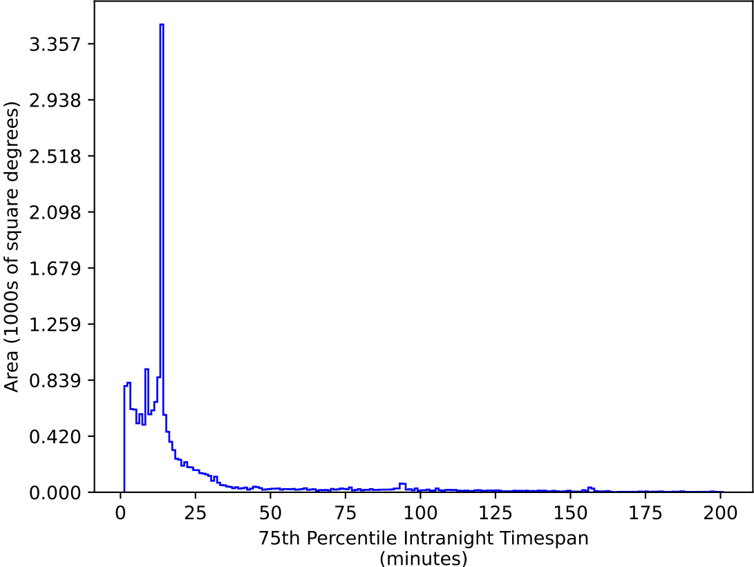
too_elab_r16_d2_ugrizy_v3.4_10yrs WFD z band: 75th Percentile Intranight Timespan
