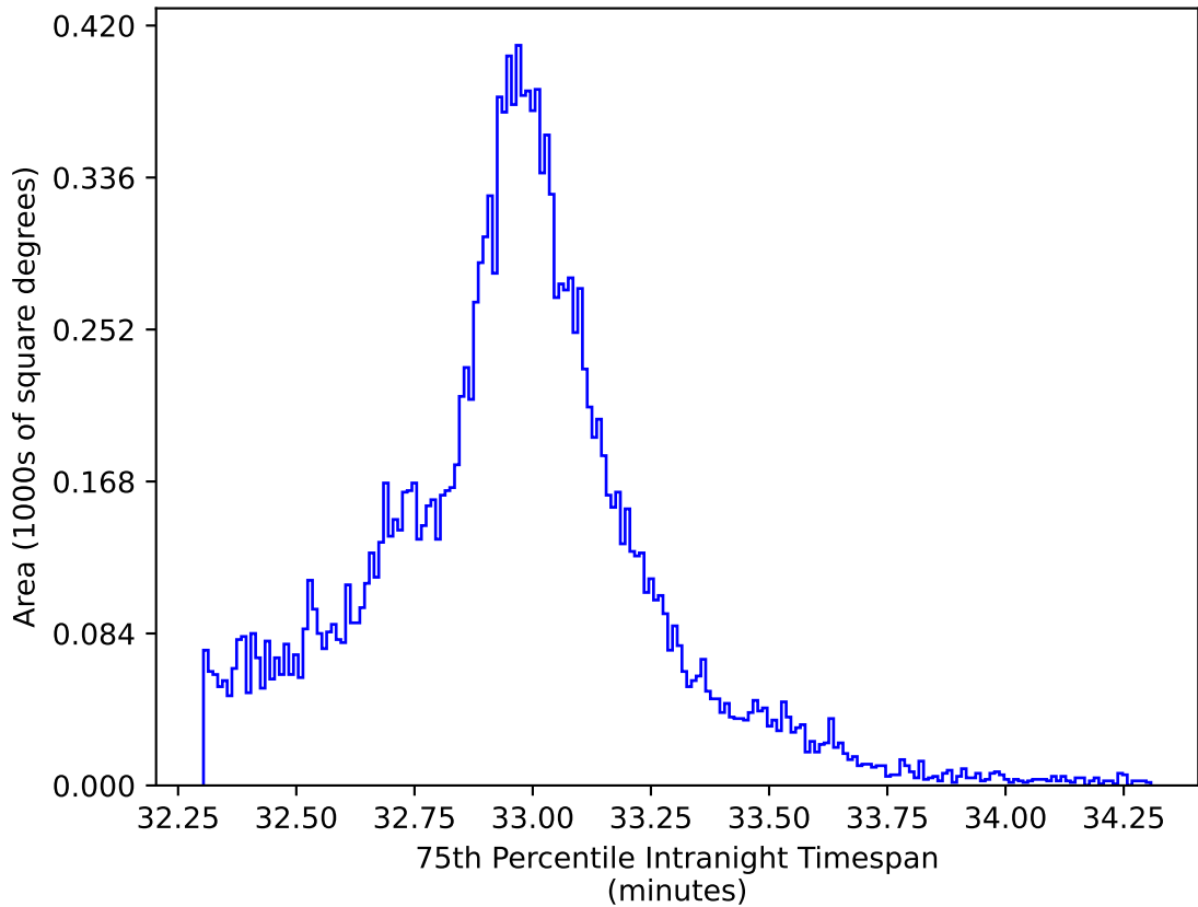
too_elab_r16_d2_ugrizy_v3.4_10yrs WFD y band: 75th Percentile Intranight Timespan
