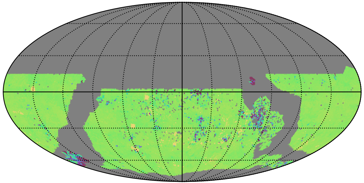
too_elab_r16_d2_ugrizy_v3.4_10yrs WFD ug bands: 75th Percentile Intranight Timespan
