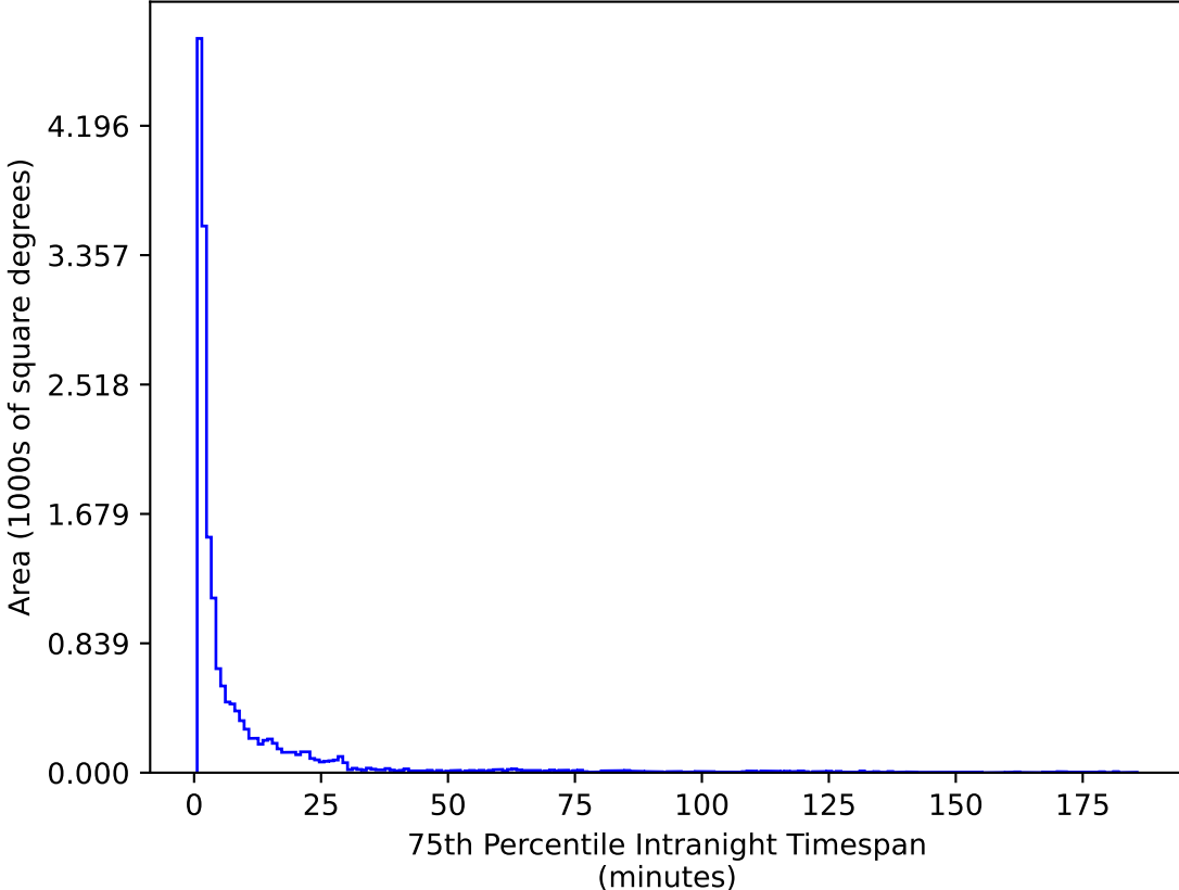
too_elab_r16_d2_ugrizy_v3.4_10yrs WFD u band: 75th Percentile Intranight Timespan
