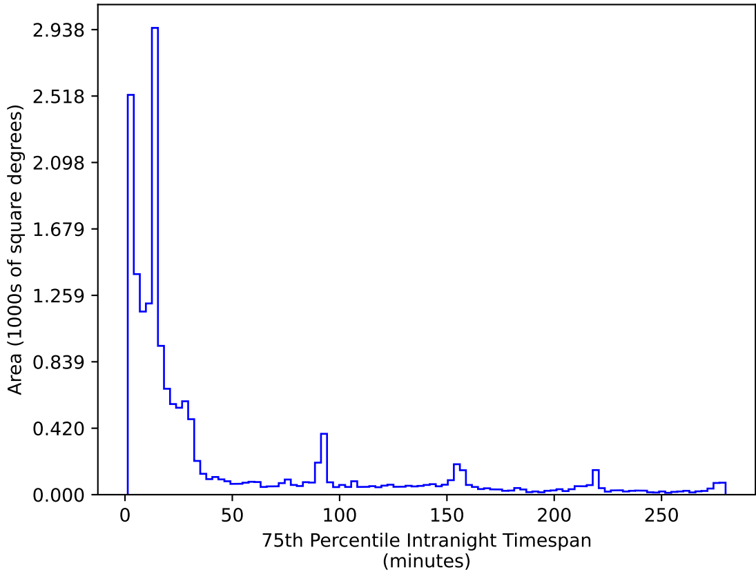
too_elab_r16_d2_ugrizy_v3.4_10yrs WFD r band: 75th Percentile Intranight Timespan
