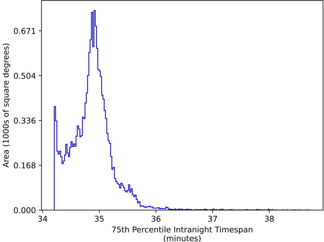
too_elab_r16_d2_ugrizy_v3.4_10yrs WFD iz bands: 75th Percentile Intranight Timespan
