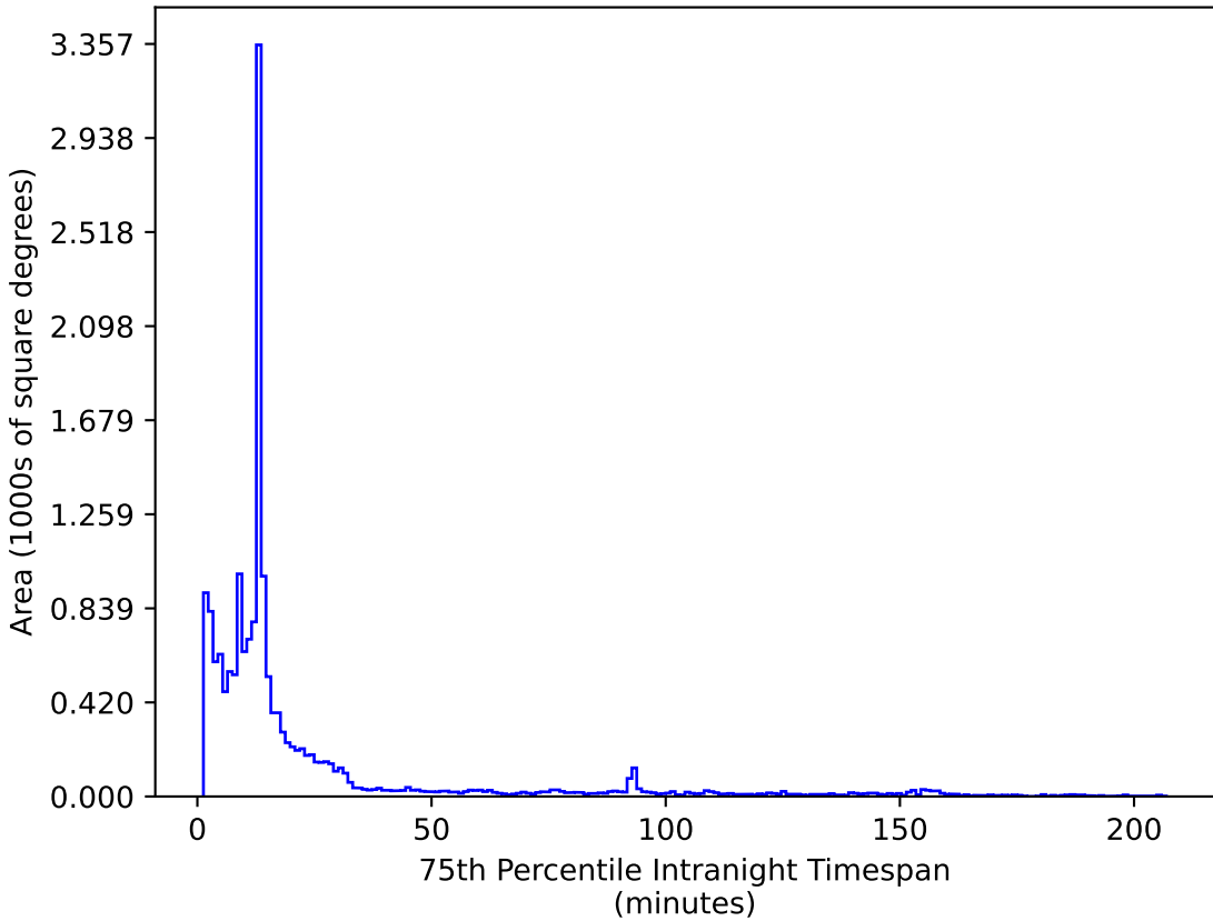
too_elab_r16_d2_ugrizy_v3.4_10yrs WFD i band: 75th Percentile Intranight Timespan
