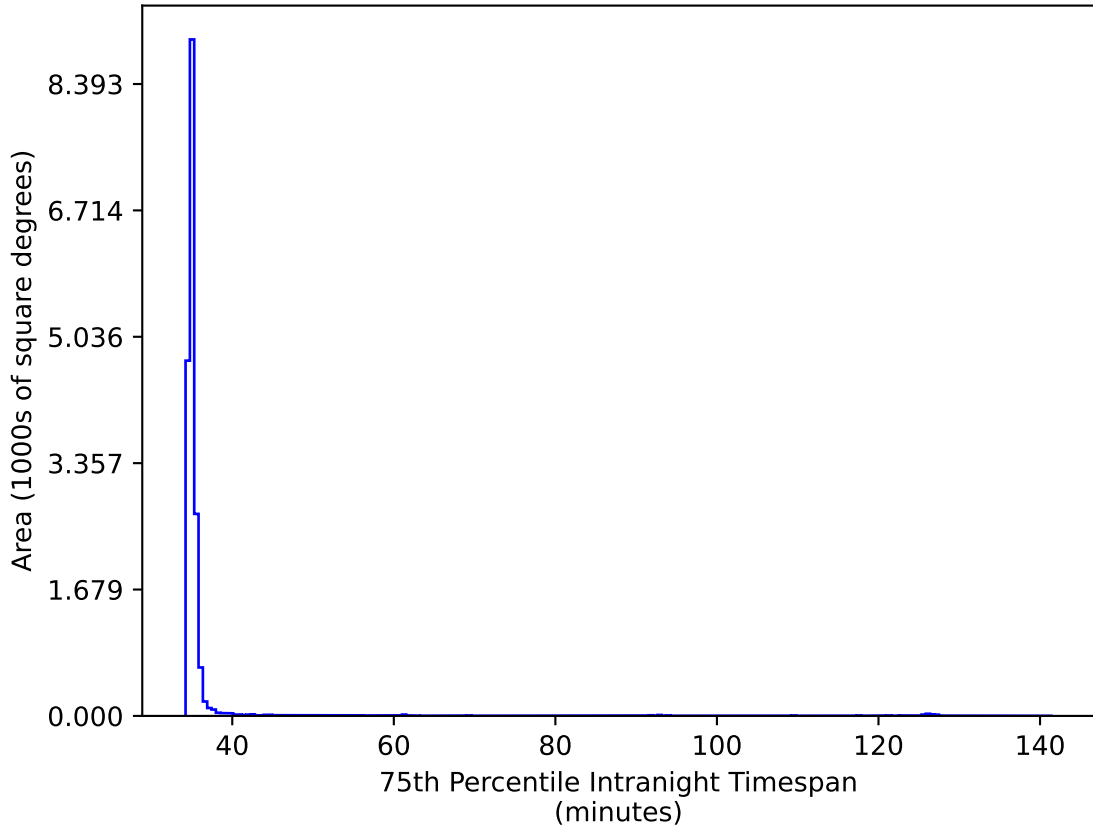
too_elab_r16_d2_ugrizy_v3.4_10yrs WFD gr bands: 75th Percentile Intranight Timespan
