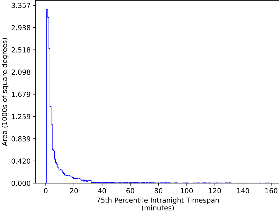
too_elab_r16_d2_ugrizy_v3.4_10yrs WFD g band: 75th Percentile Intranight Timespan
