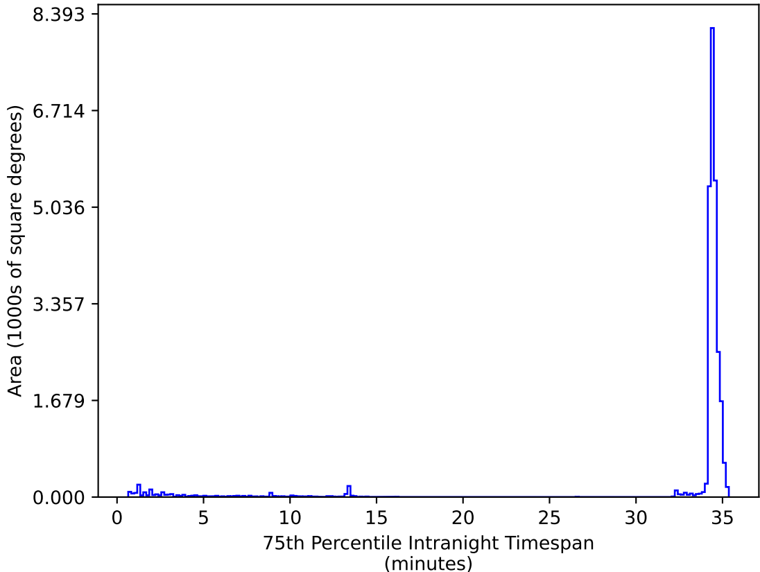
too_elab_r16_d2_ugrizy_v3.4_10yrs All sky zy bands: 75th Percentile Intranight Timespan
