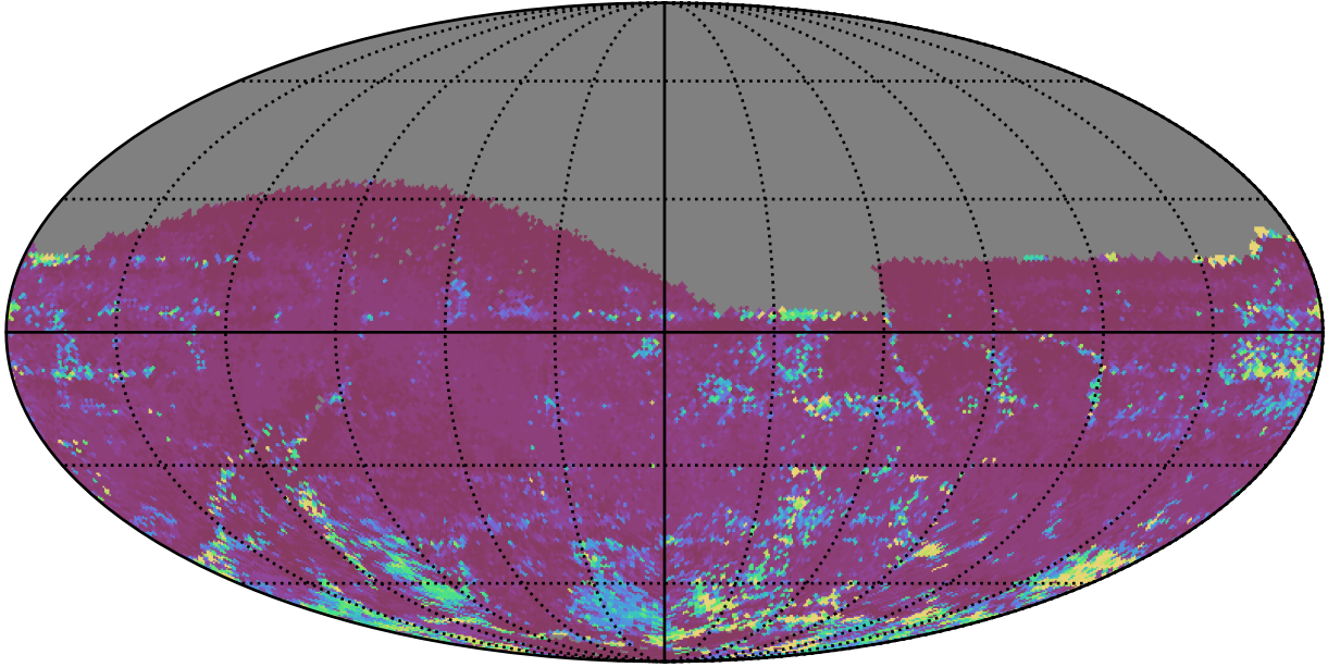
too_elab_r16_d2_ugrizy_v3.4_10yrs All sky z band: 75th Percentile Intranight Timespan
