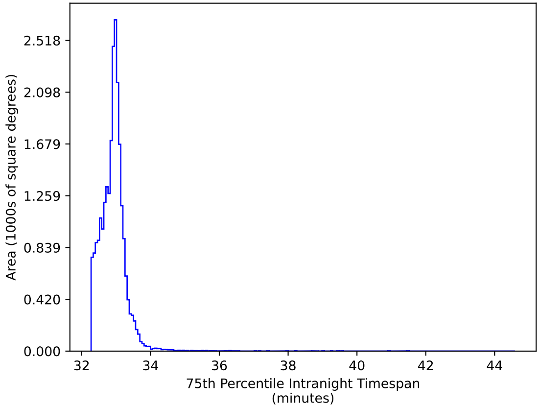
too_elab_r16_d2_ugrizy_v3.4_10yrs All sky y band: 75th Percentile Intranight Timespan
