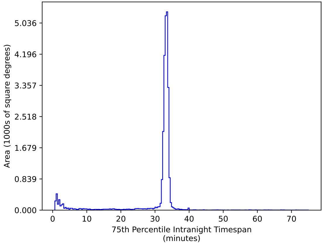
too_elab_r16_d2_ugrizy_v3.4_10yrs All sky ug bands: 75th Percentile Intranight Timespan
