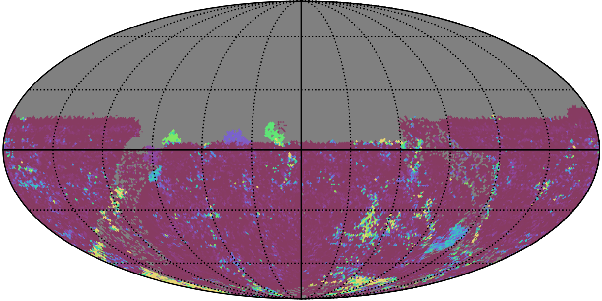
too_elab_r16_d2_ugrizy_v3.4_10yrs All sky u band: 75th Percentile Intranight Timespan
