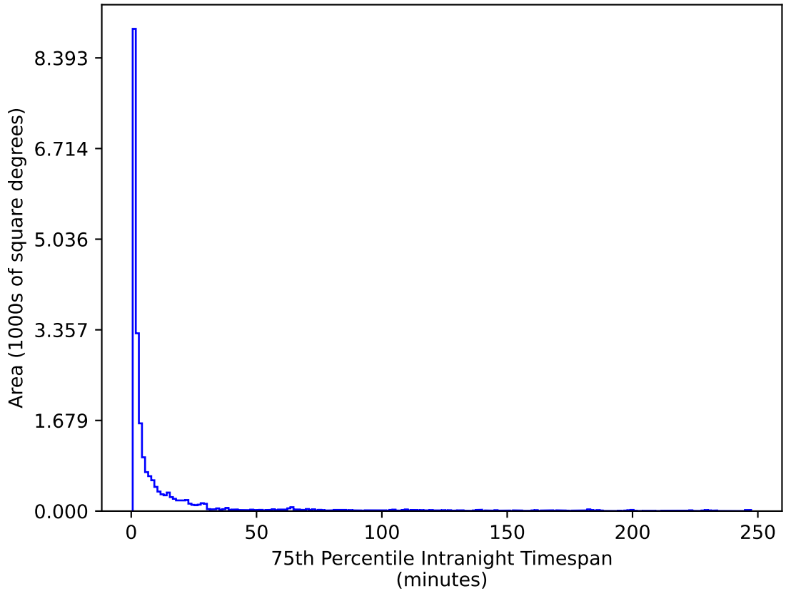
too_elab_r16_d2_ugrizy_v3.4_10yrs All sky u band: 75th Percentile Intranight Timespan
