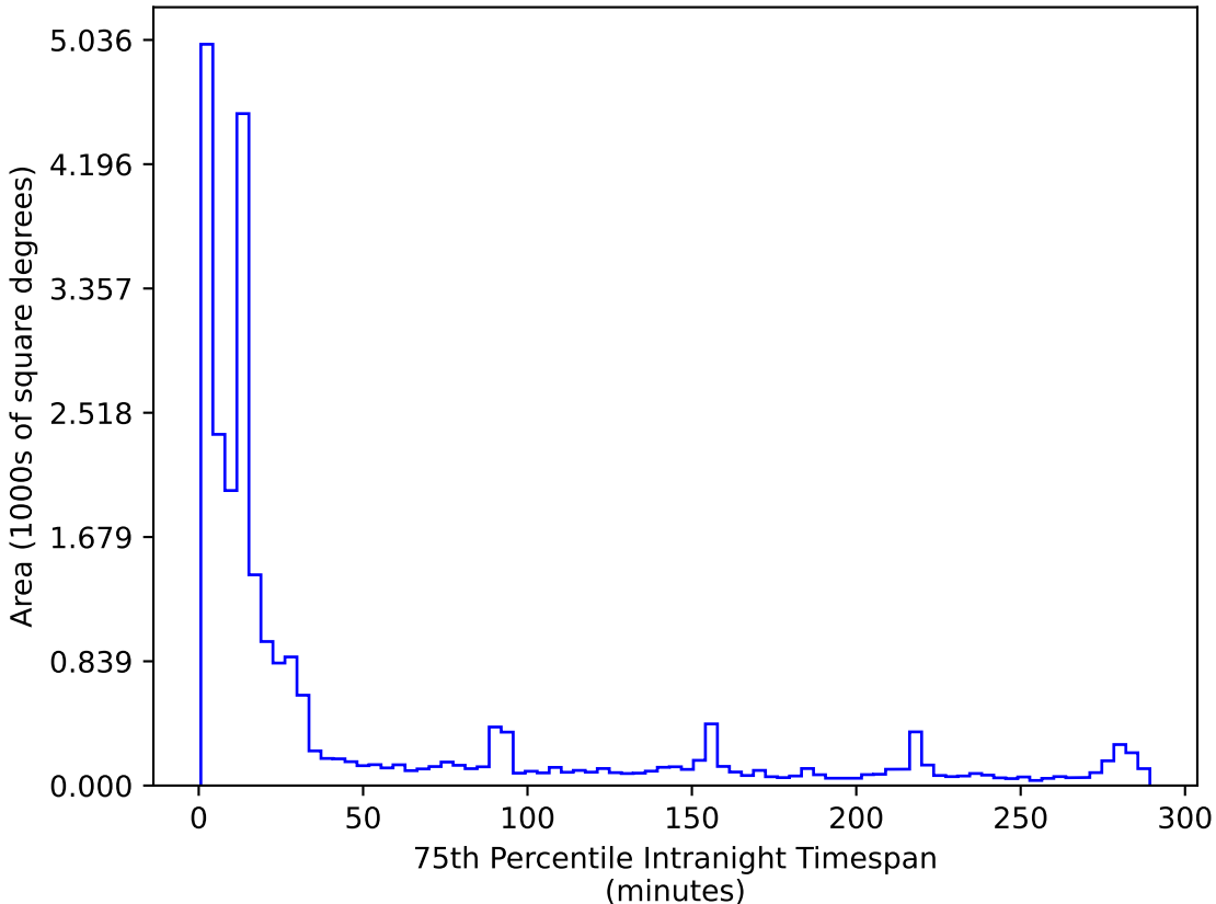
too_elab_r16_d2_ugrizy_v3.4_10yrs All sky r band: 75th Percentile Intranight Timespan
