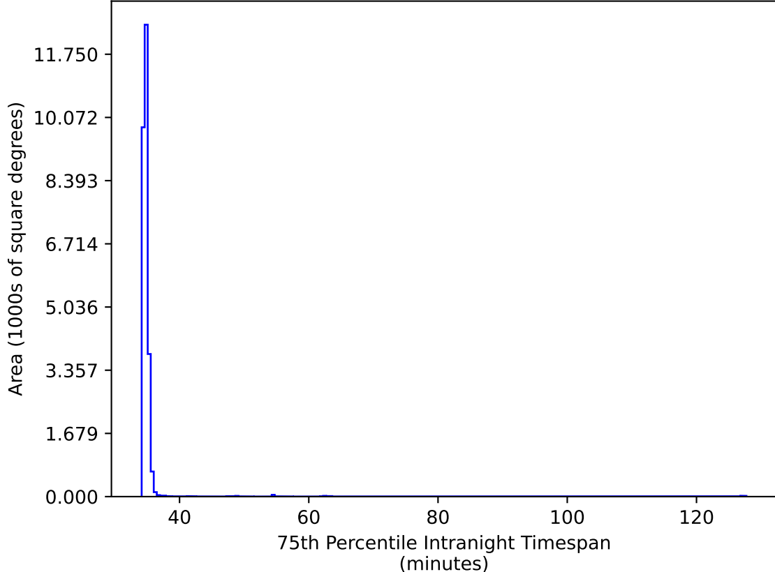
too_elab_r16_d2_ugrizy_v3.4_10yrs All sky iz bands: 75th Percentile Intranight Timespan
