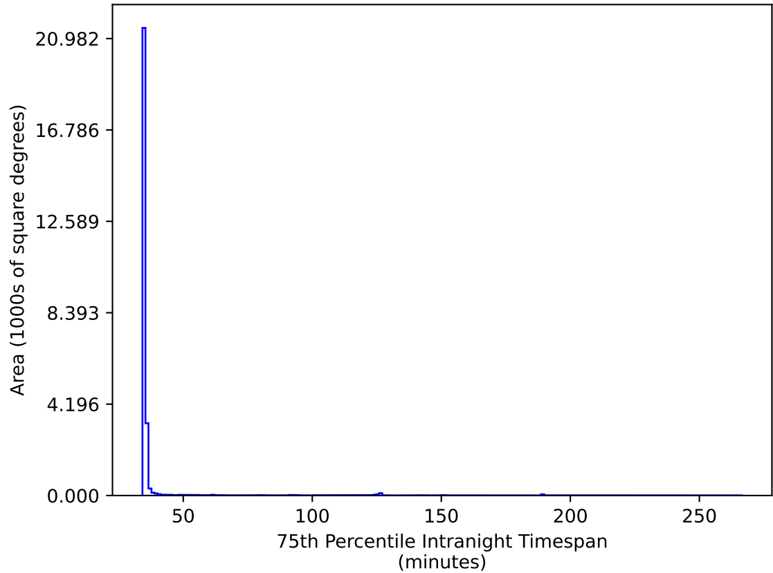
too_elab_r16_d2_ugrizy_v3.4_10yrs All sky gr bands: 75th Percentile Intranight Timespan
