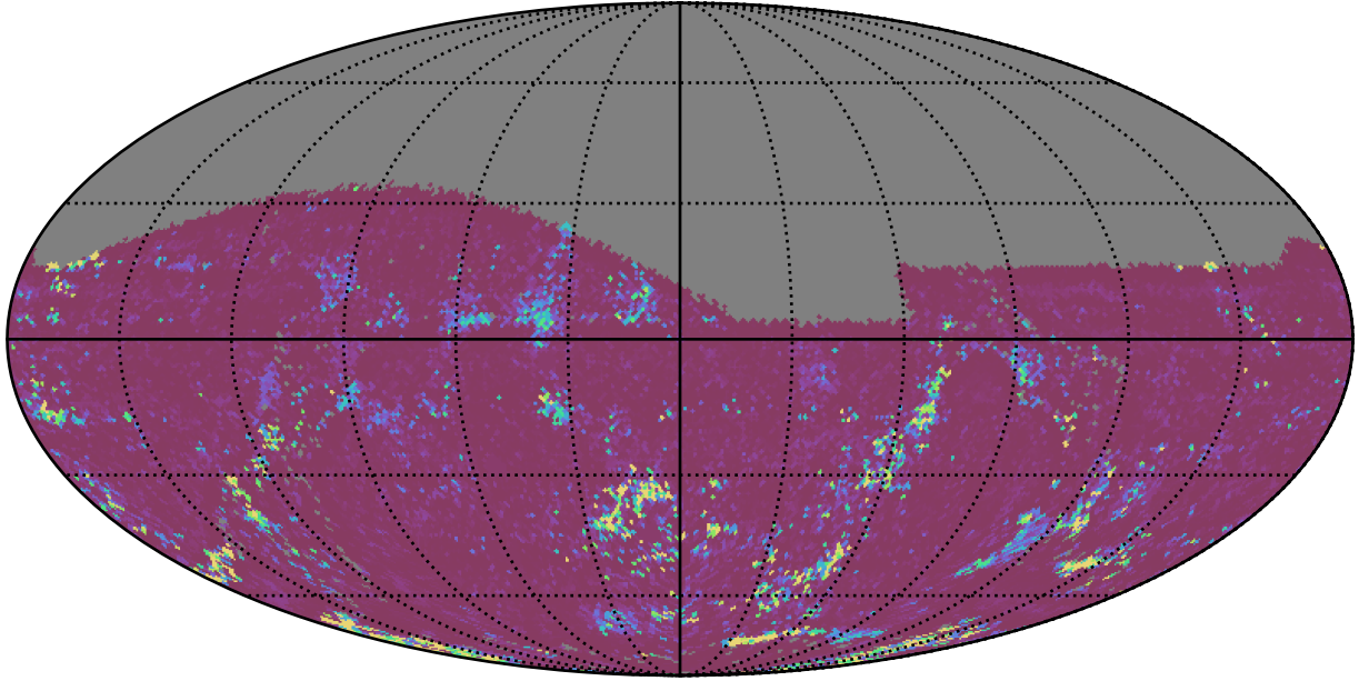
too_elab_r16_d2_ugrizy_v3.4_10yrs All sky g band: 75th Percentile Intranight Timespan
