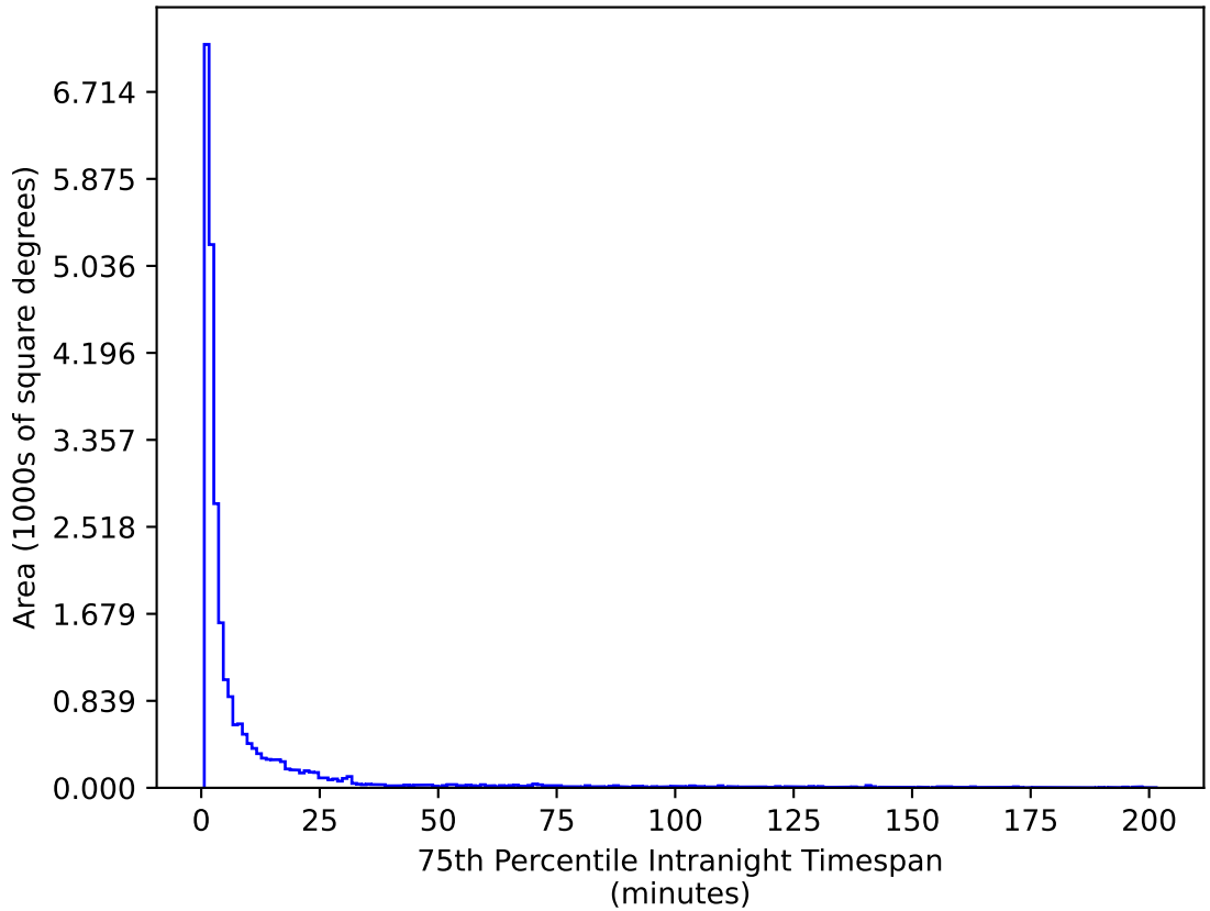
too_elab_r16_d2_ugrizy_v3.4_10yrs All sky g band: 75th Percentile Intranight Timespan
