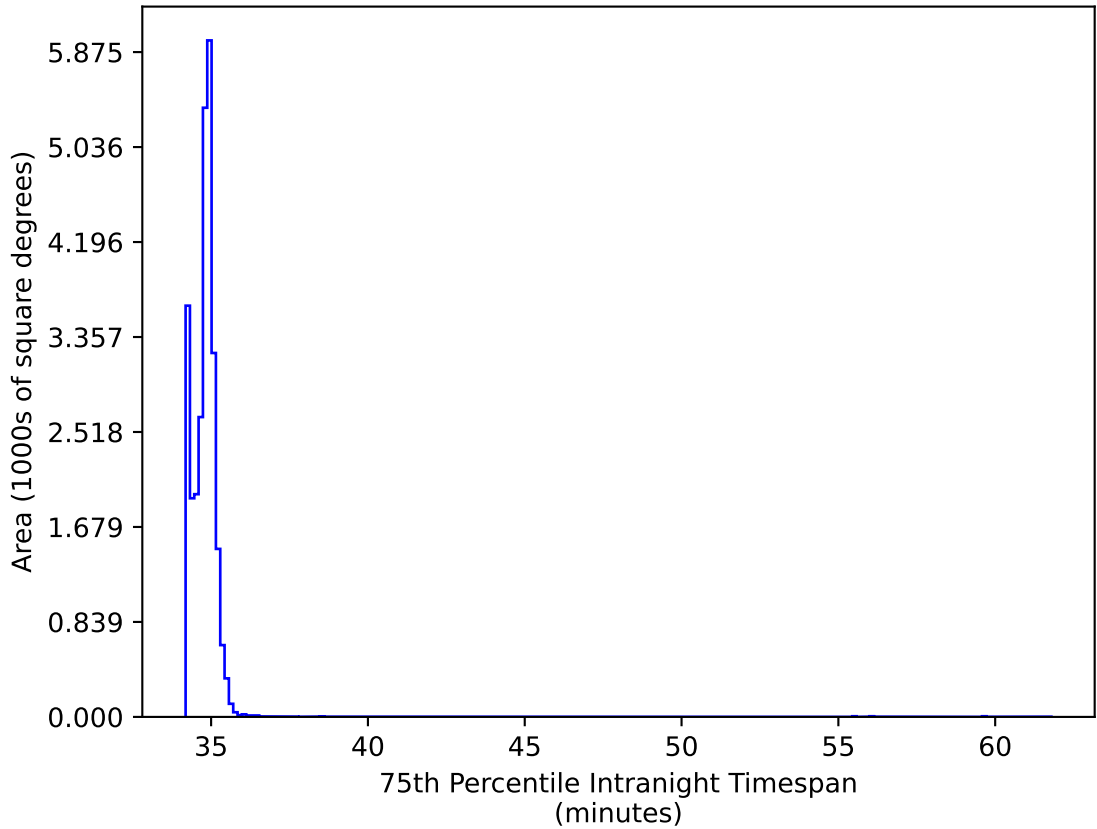
too_elab_r16_d2_ugrizy_v3.4_10yrs All sky all bands: 75th Percentile Intranight Timespan
