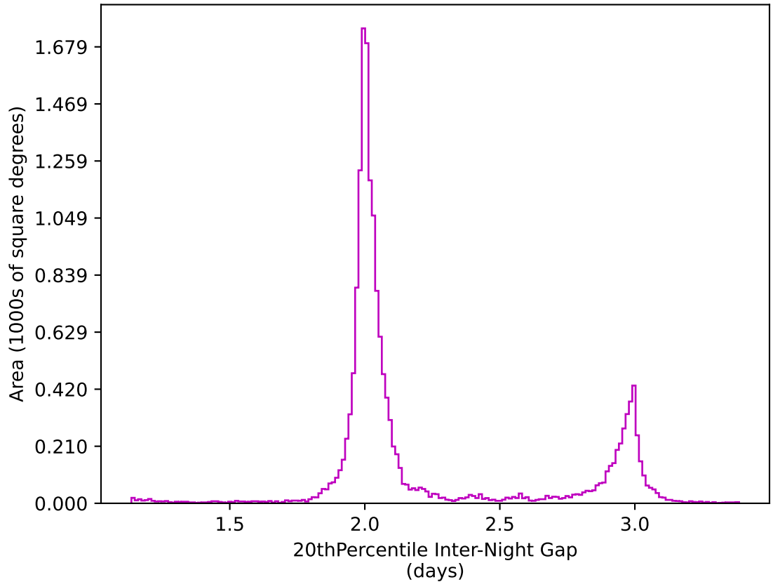
too_elab_r16_d2_ugrizy_v3.4_10yrs WFD z band: 20thPercentile Inter-Night Gap
