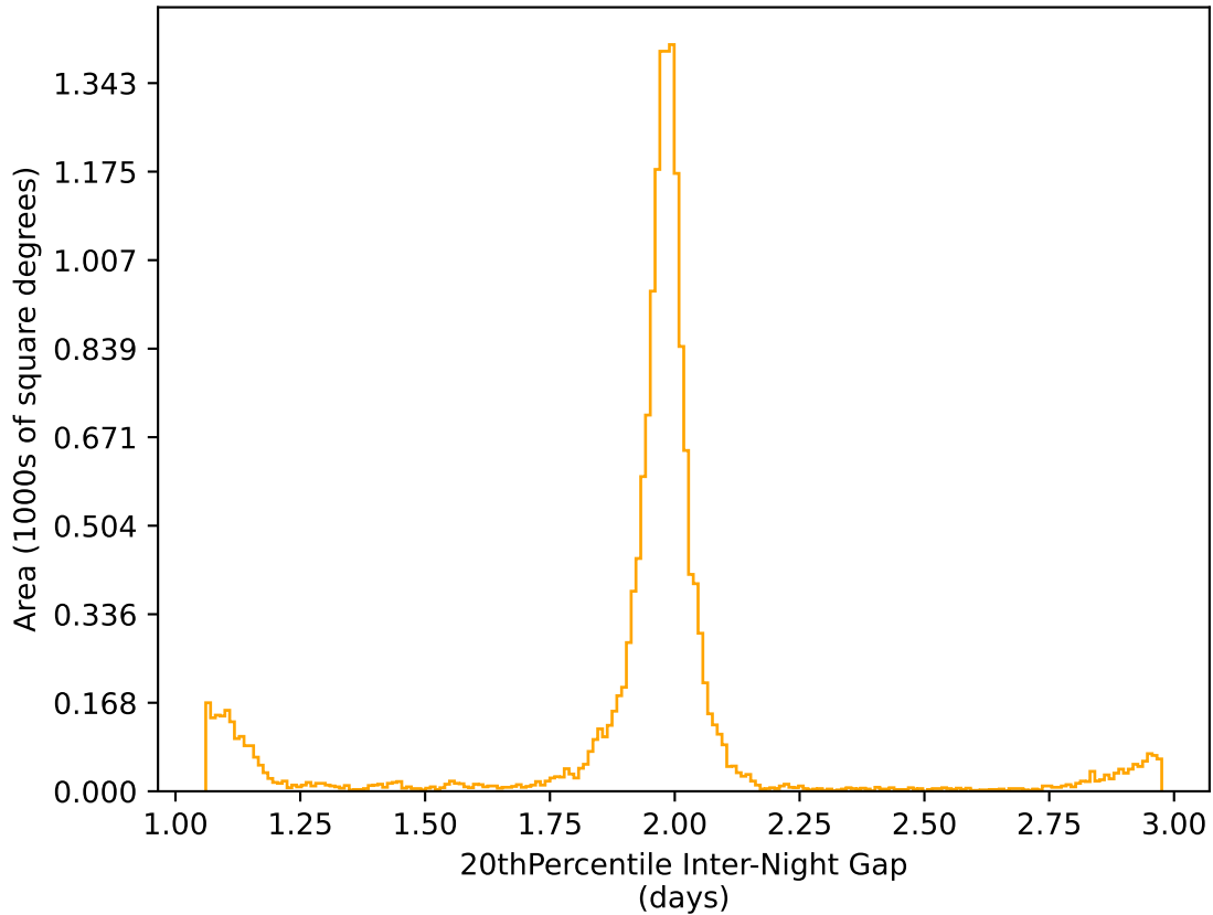
too_elab_r16_d2_ugrizy_v3.4_10yrs WFD r band: 20thPercentile Inter-Night Gap
